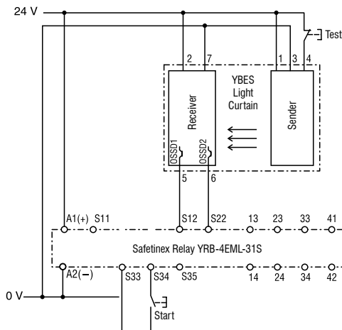
FIG. 25: CONNECTION DIAGRAM FOR MANUAL RESTART MODE
