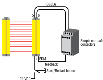
FIG. 32: CONNECTION OF LIGHT CURTAIN WITH EDM TURNED ON AND MANUAL RESTART SELECTED
