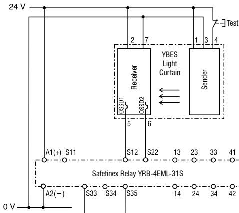
FIG. 26: CONNECTION DIAGRAM FOR AUTOMATIC RESTART MODE
