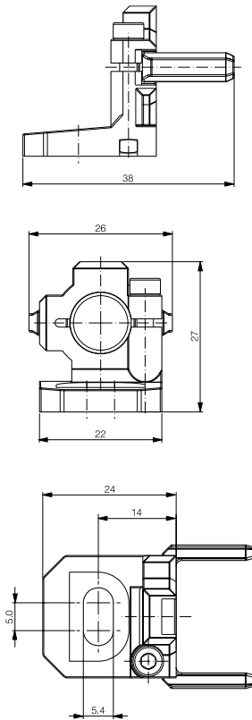
FIG. 17.1: STANDARD TOP/BOTTOM MOUNTING BRACKET No. 5 (REF: YXW-0005-000)
