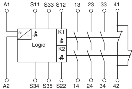
FIG. 23: BLOCK DIAGRAM
