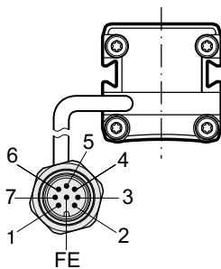
FIG. 21: M12 PIN ASSIGNMENT (RECEIVER)
