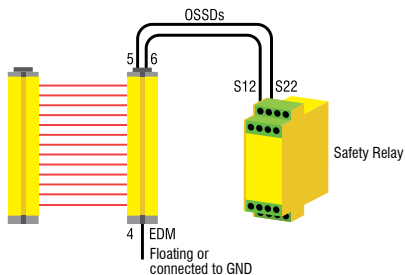
FIG. 29: CONNECTION WITH EDM DEACTIVATED
