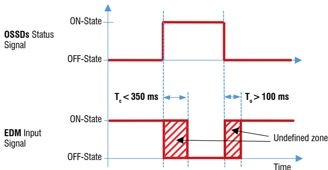
FIG. 30: EDM INPUT SIGNAL TIMING DIAGRAM
