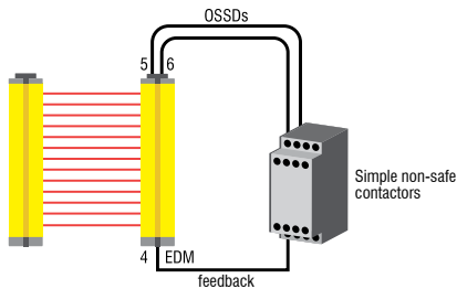
FIG. 28: CONNECTION WITH EDM ACTIVATED
