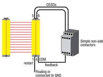
FIG. 31: CONNECTION OF LIGHT CURTAIN WITH EDM TURNED ON AND AUTOMATIC RESTART SELECTED
