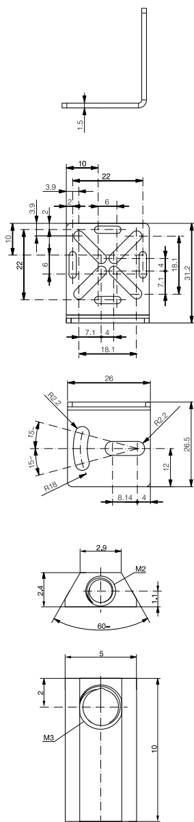
FIG. 19.1: TOP AND BOTTOM OPTIONAL MOUNTING BRACKET No. 7 (REF: YXW-0007-000)
