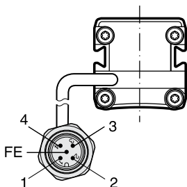
FIG. 20: M12 PIN ASSIGNMENT (SENDER)
